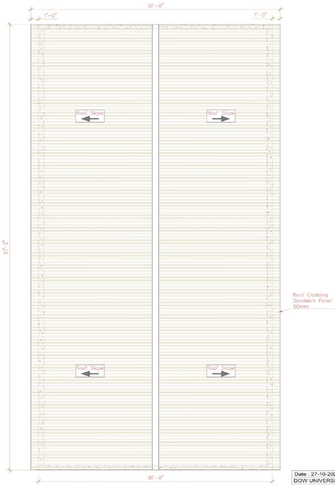
ROOF SHEETING PLAN
